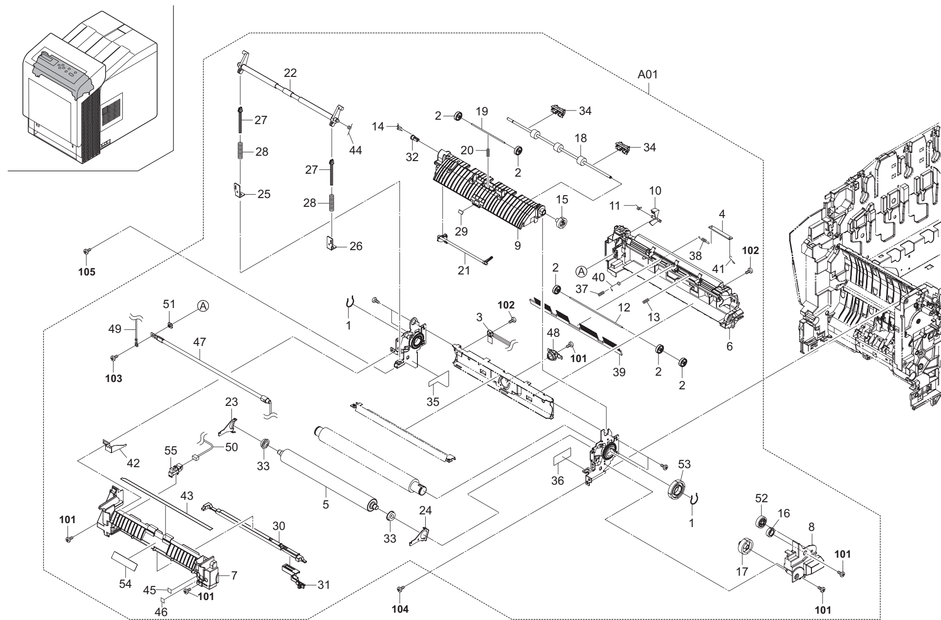
FIG. 11 Fuser Section
