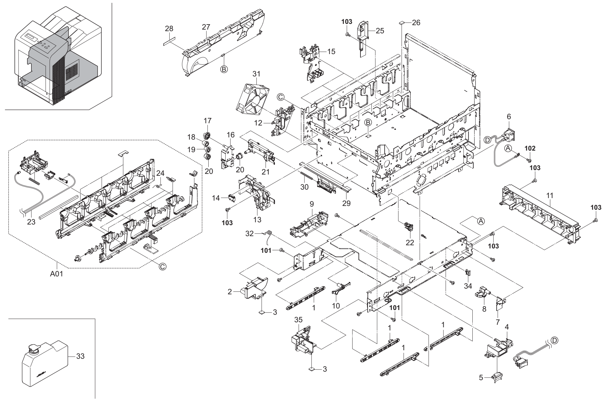
FIG. 4 Frames 2 (21/23ppm 250sheet)
